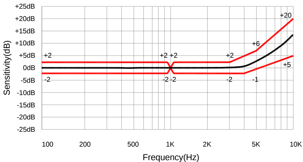
Frequency Response (0dB=1V/Pa)
